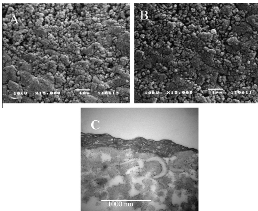
Figure 6. Panels A and B: SEM images of Tyro/E-LbL at a higher magnification ( \times 15,000 ) at time zero (panel A) and after two months (panel B) upon storage at 4^{\circ}\text{C} . Panel C: TEM image of a section of Tyro/E-LbL particle upon storage for two months at 4^{\circ}\text{C} . LbL layers are clearly visible in the upper part of the picture.
